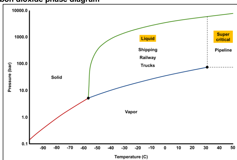
Figure 13: Carbon dioxide phase diagram
