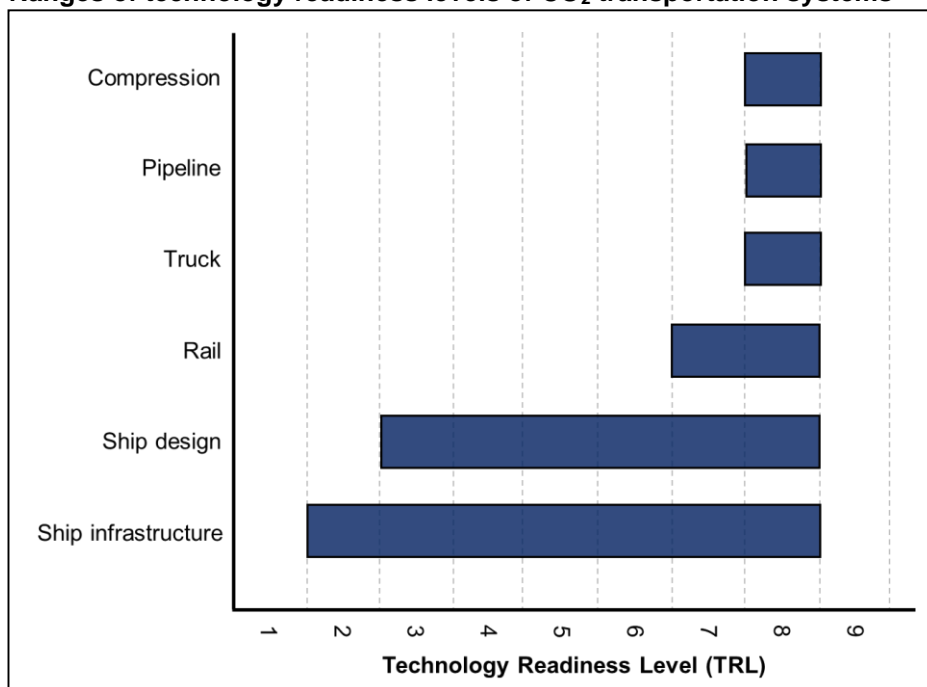
Figure 15: Ranges of technology readiness levels of CO 2 transportation systems
