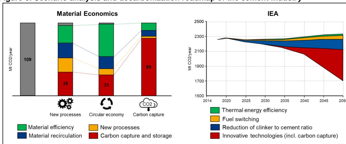
Figure 6: Scenario analysis and decarbonization roadmap of the cement industry
