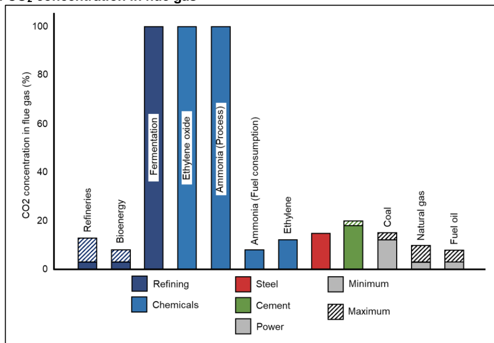
Figure 8: CO 2 concentration in flue gas
