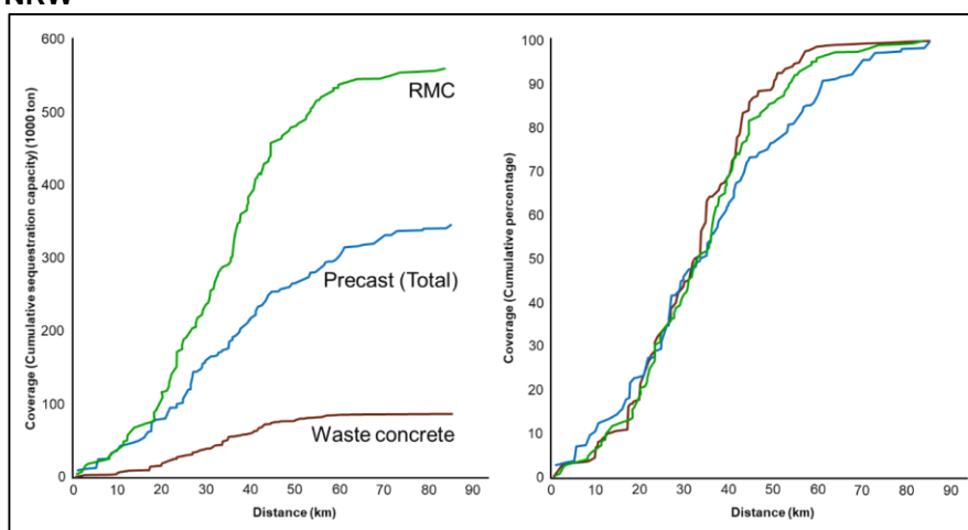
Figure 21: The relationship between distance and sequestration capacities of cementitious materials in NRW
