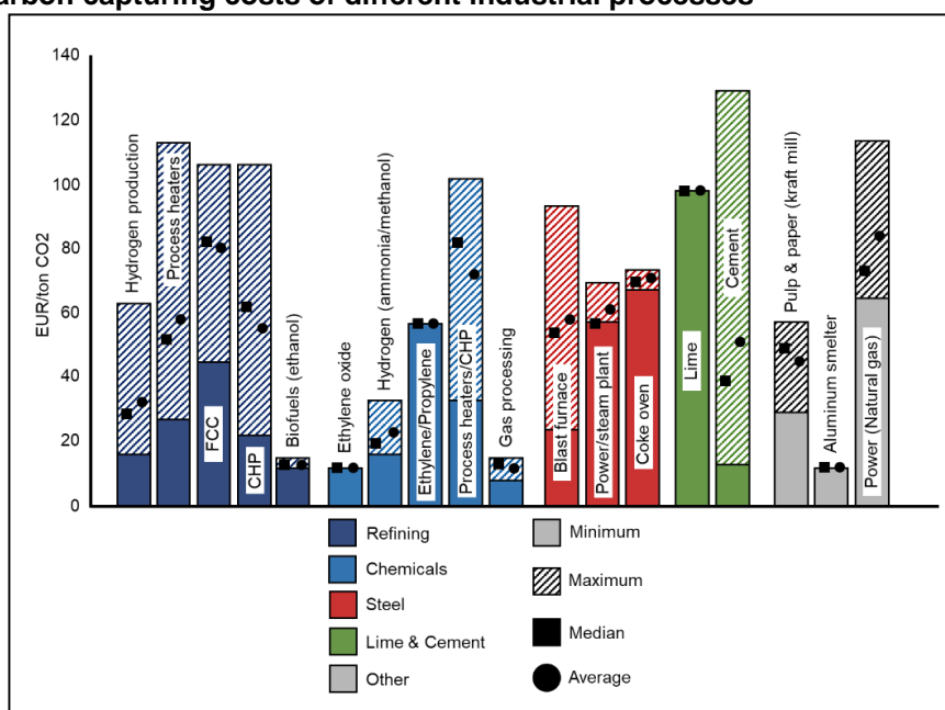
Figure 10: Carbon capturing costs of different industrial processes
