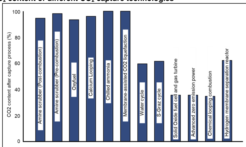
Figure 12: CO 2 content of different CO 2 capture technologies
