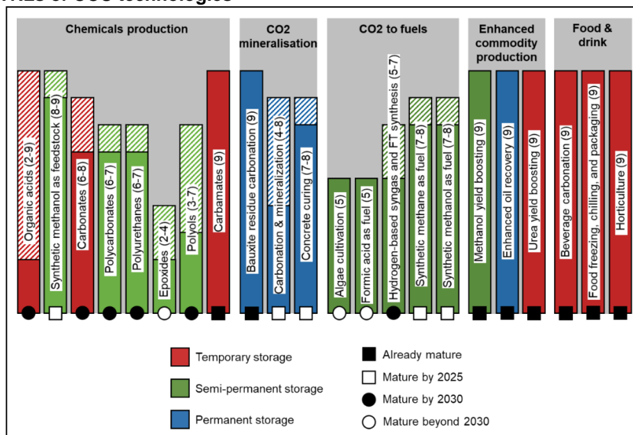
Figure 20: TRLs of CCU technologies
