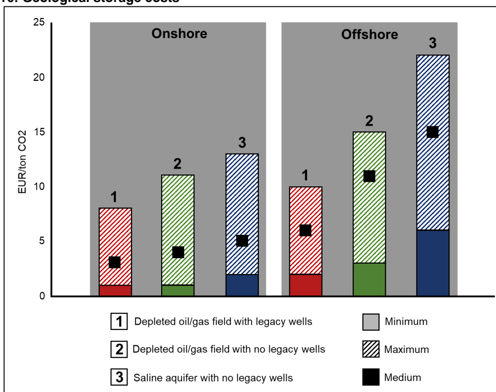
Figure 16: Geological storage costs
