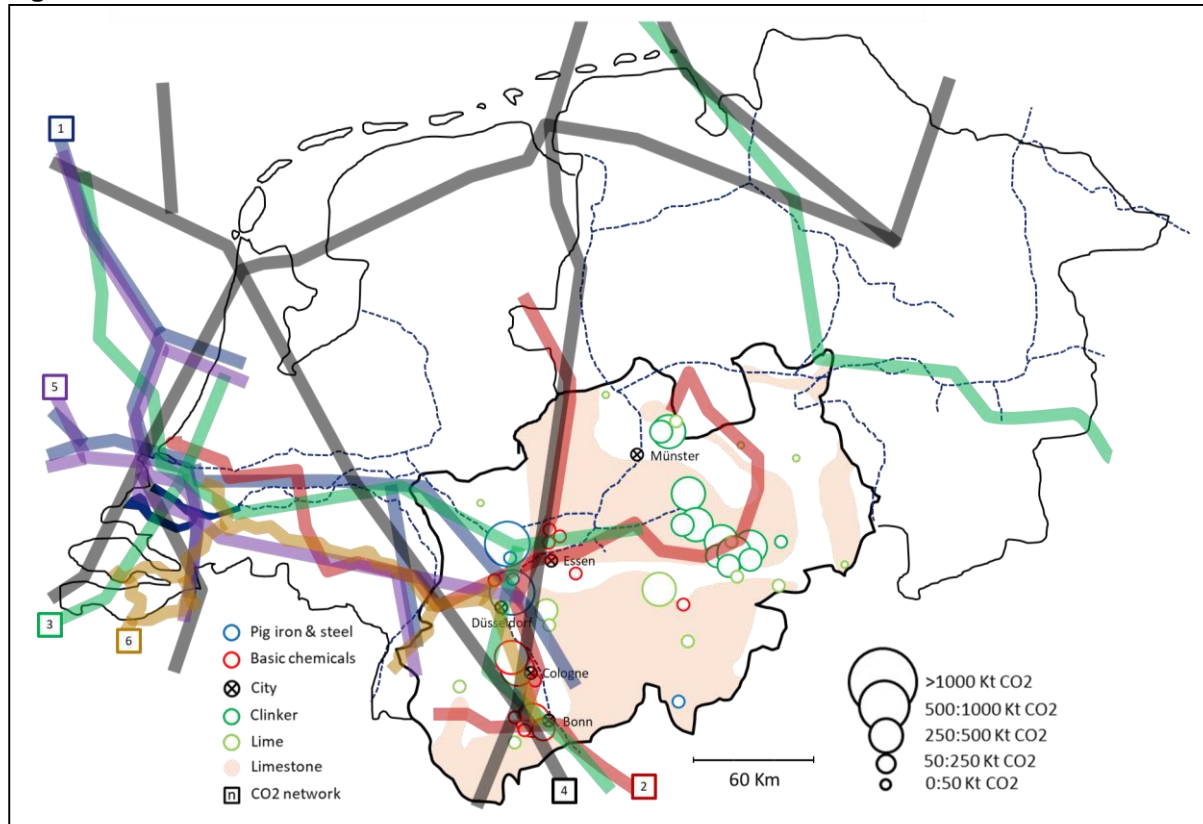
Figure 19: Potential CO 2 networks in NRW
