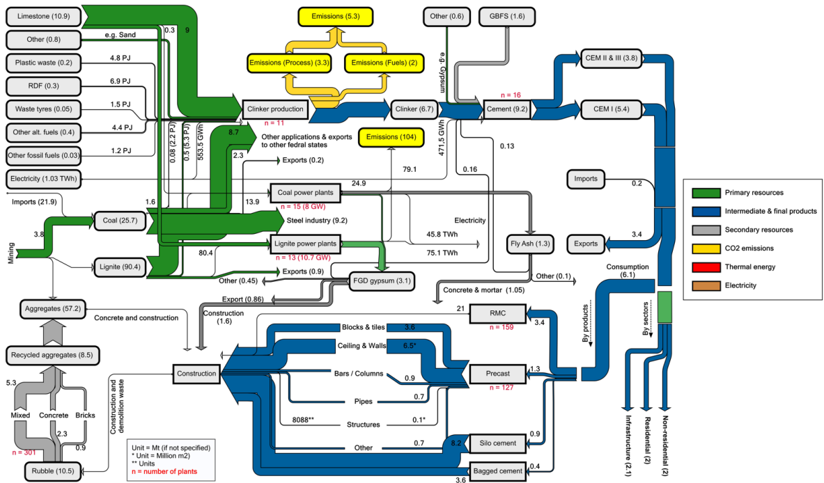
Figure 2: MFA model of cement and construction industries in NRW
