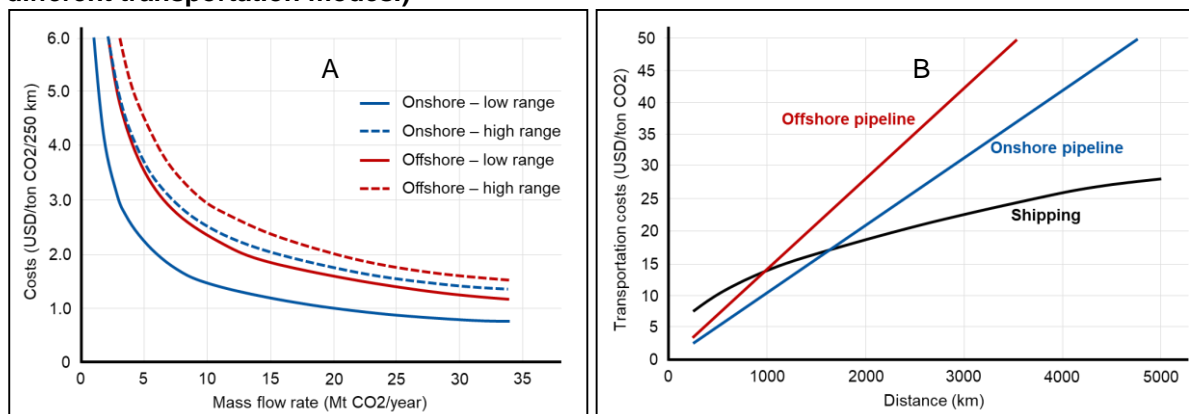
Figure 14: CO 2 transportation costs (A: flow rate of pipeline vs. costs. B: distance vs. costs of different transportation modes.)
