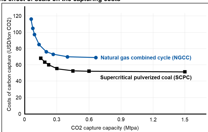
Figure 11: The effect of scale on the capturing costs
